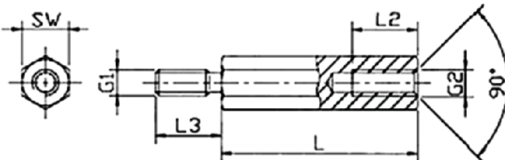
Thread Lengths (mm)
