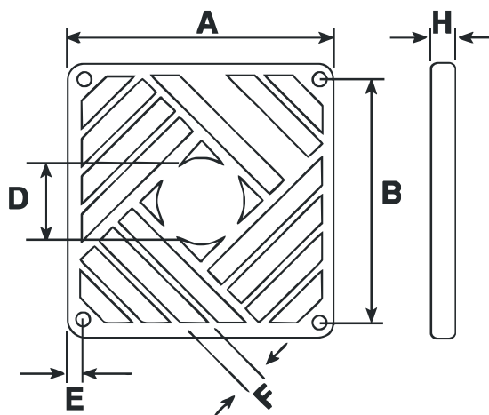
FINGER GUARD
