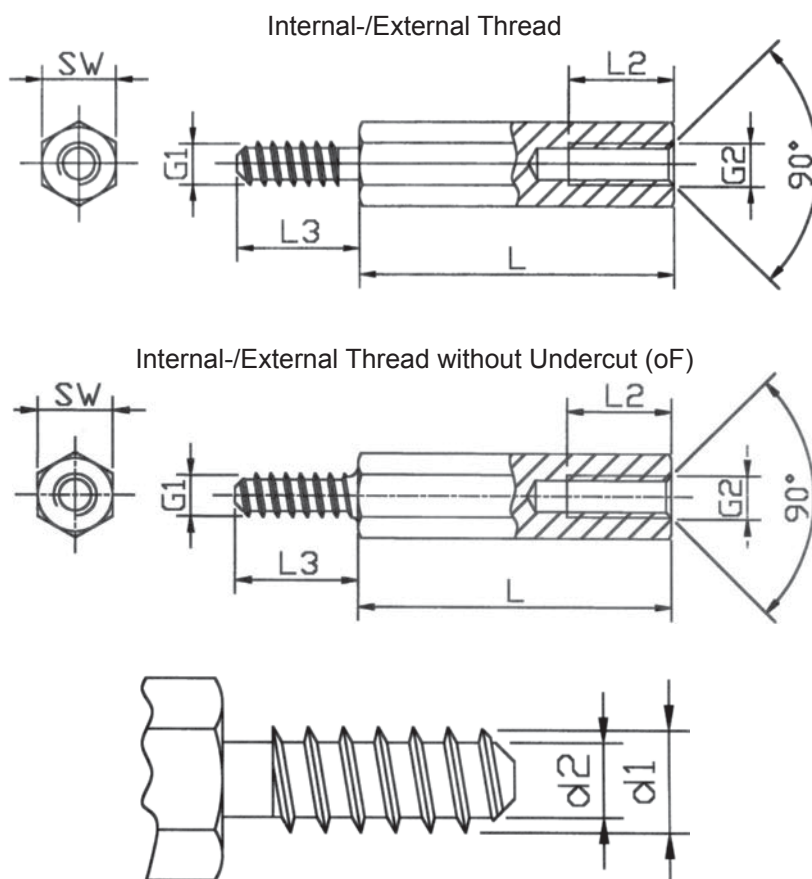
Internal Thread G2
