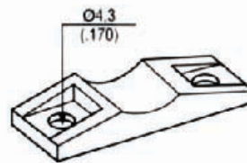
■ MOUNT-B for KB-09
