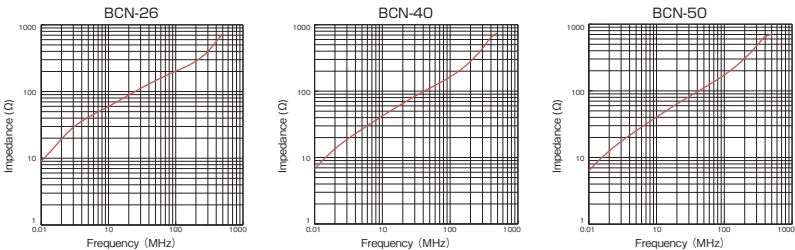
Impedance vs frequency
