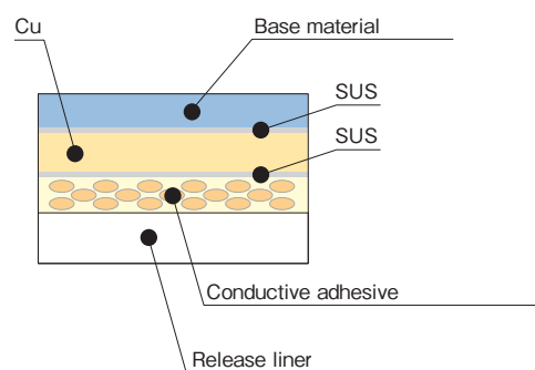
REMI-FA/-AC (Adhesive layer conductive type)
