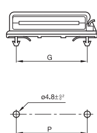
Snap on type mounting hole and pitch
