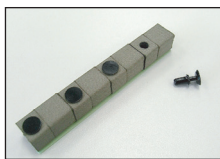
Punching+ Rivet processing
