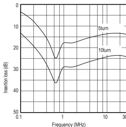
Insertion loss frequency properties*
