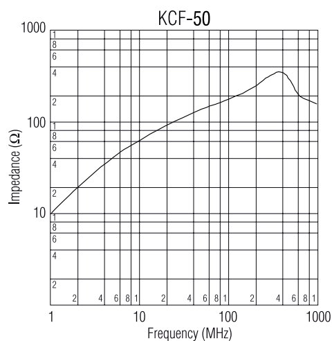
Impedance vs frequency properties*
